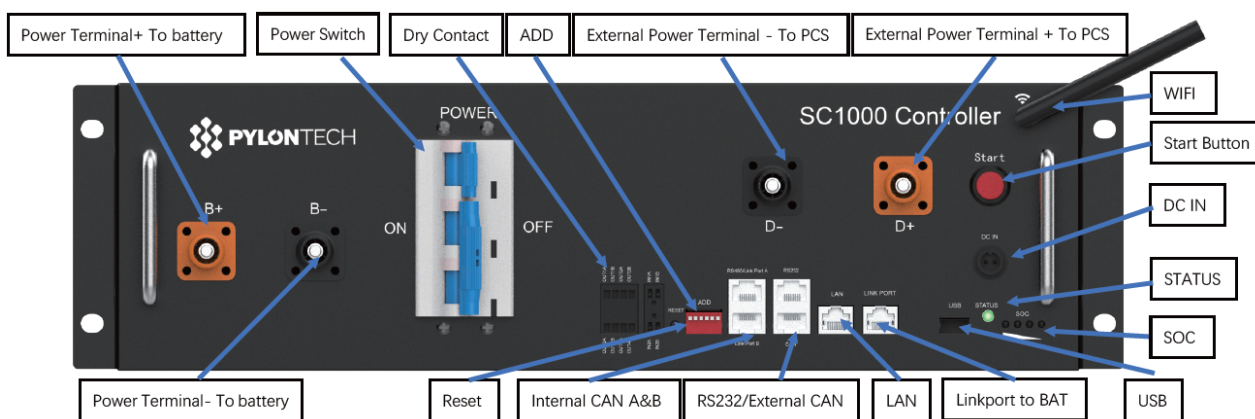
Figura 29 – BMS SC1000 Wifi/USB
